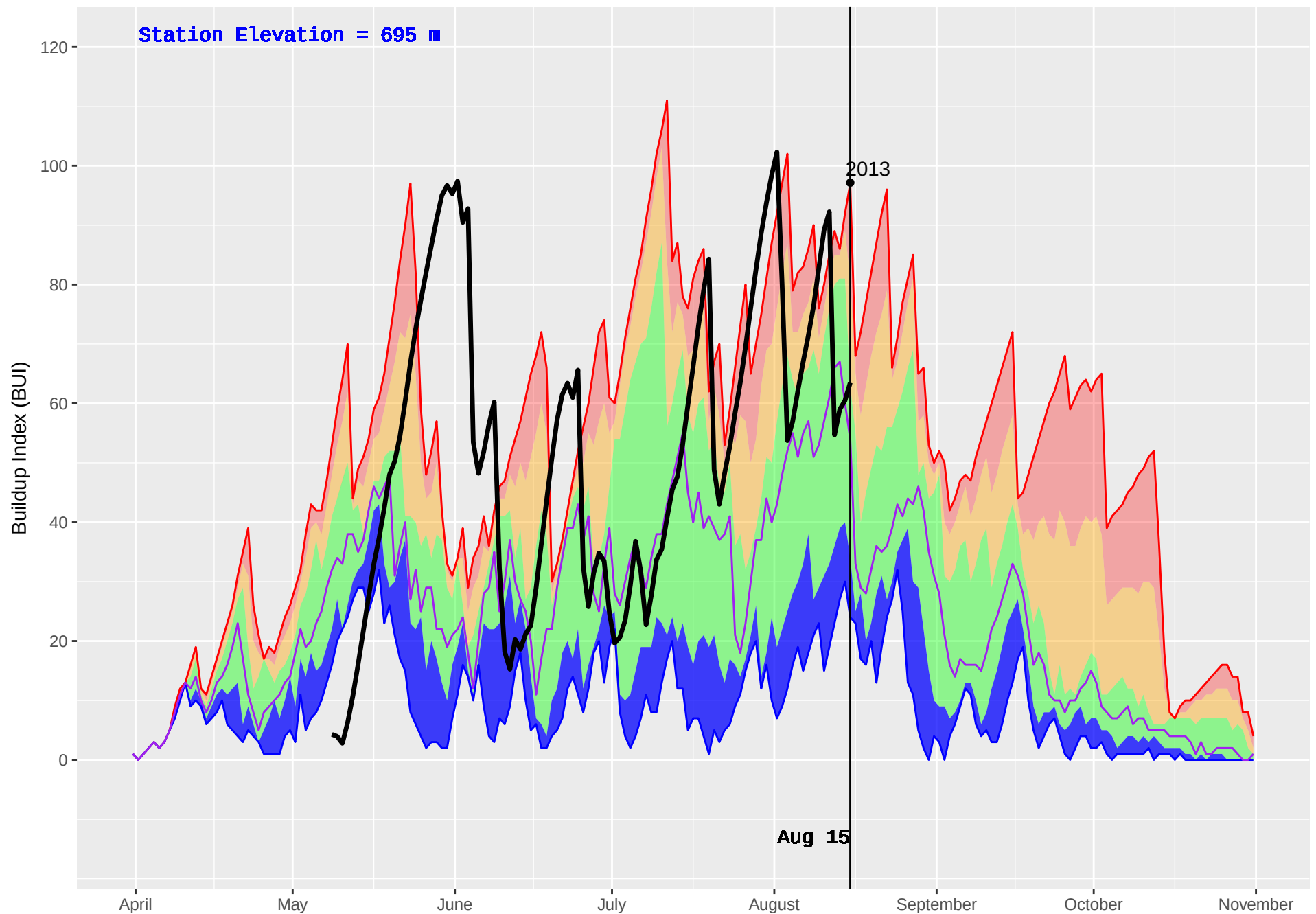
BLUE RIVER 2 (1108) : Historical (2011–2016) and Current (2018) Daily Buildup Index (BUI)
