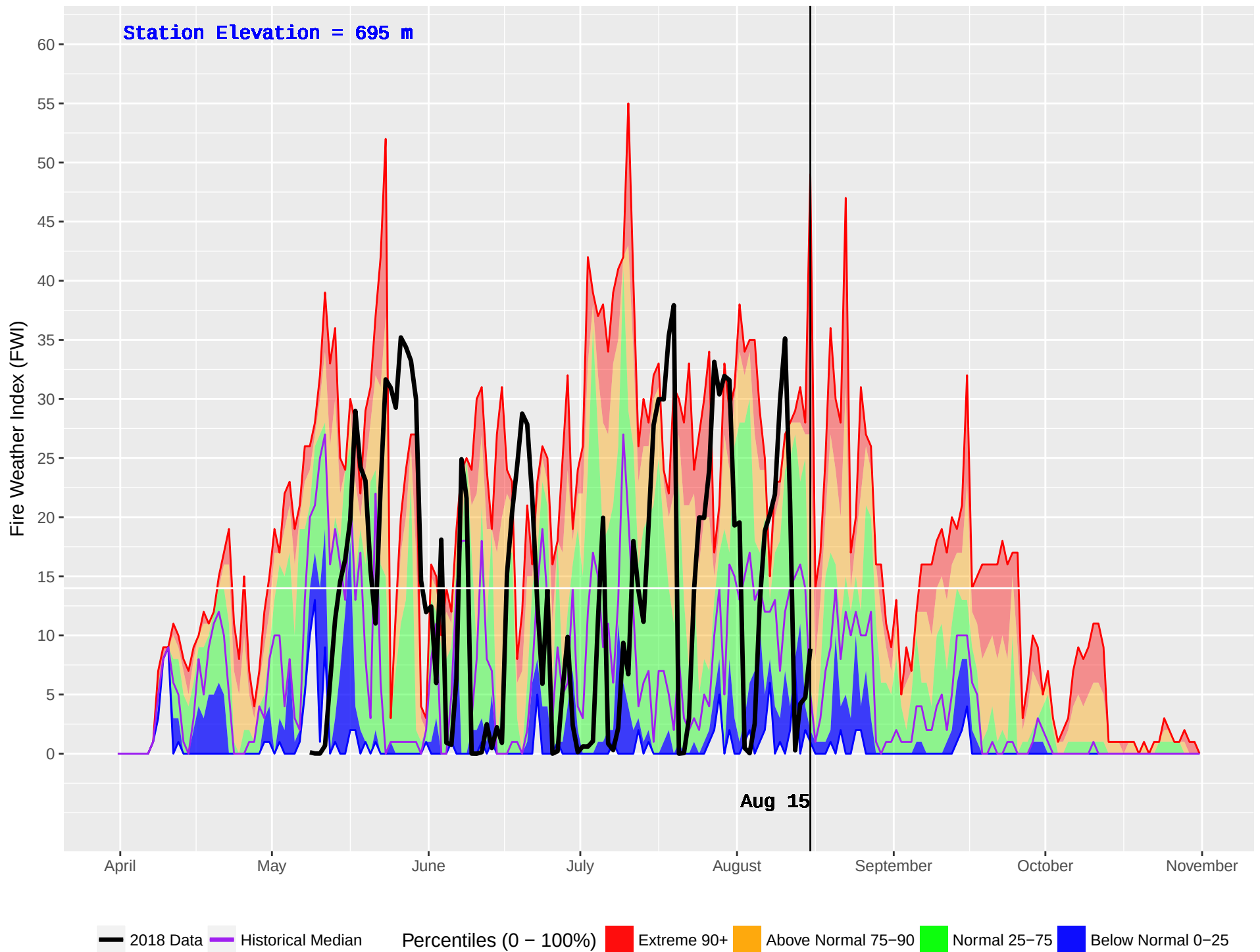
BLUE RIVER 2 (1108) : Historical (2011–2016) and Current (2018) Daily Fire Weather Index (FWI)
